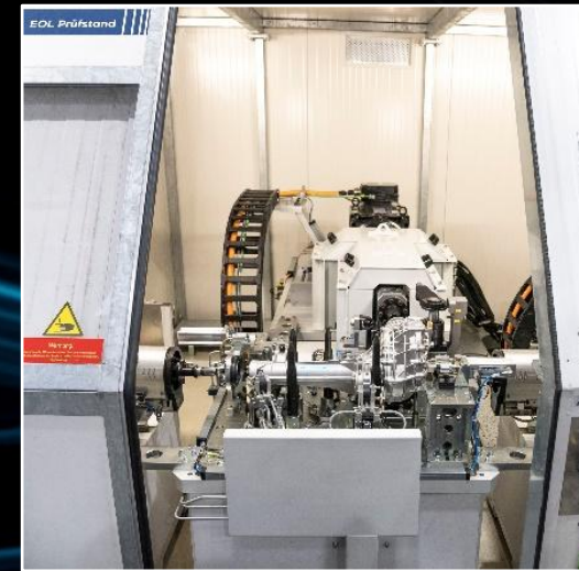
End-of-Line Testing
